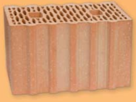
KMB PROFIBLOK 400 / BRUS 247x400x238 / 247x400x249
